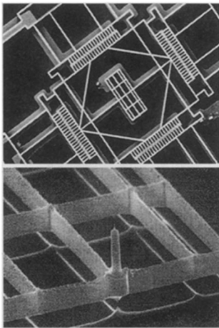
Top view of a micro-STM showing four "finger" motors surrounding a rectangular framework that carries the scanning needle (top). Close-up of needle, 5 micrometers tall (bottom).
